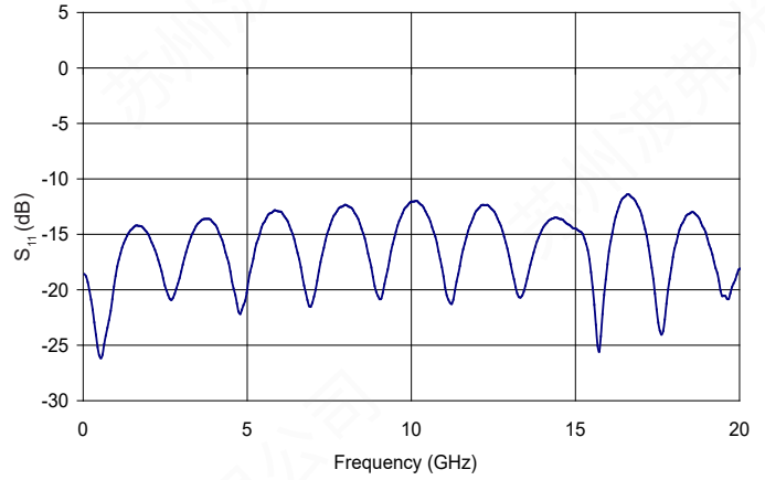
Typical S_{11} Curve
