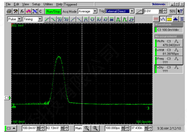
Generated 80 ps Optical Pulse
