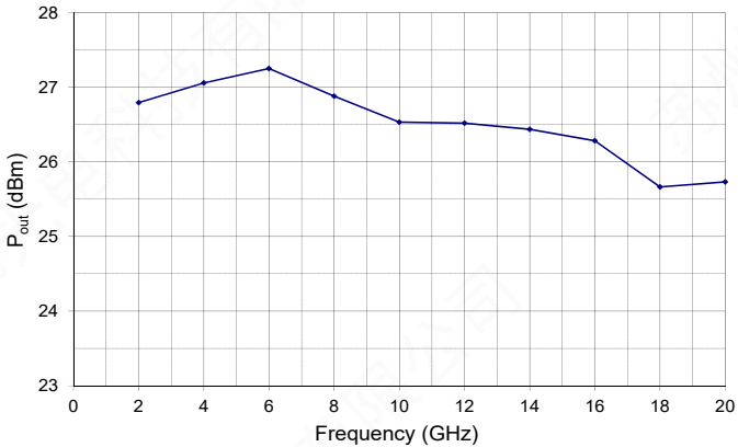
P_{out} @ 1dB Compression Curve
