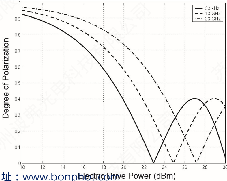
Simulated degree of polarization vs electrical power
